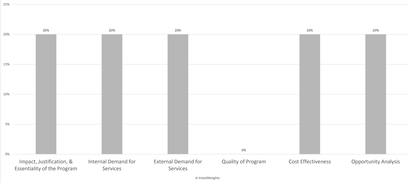
Weight Medians
